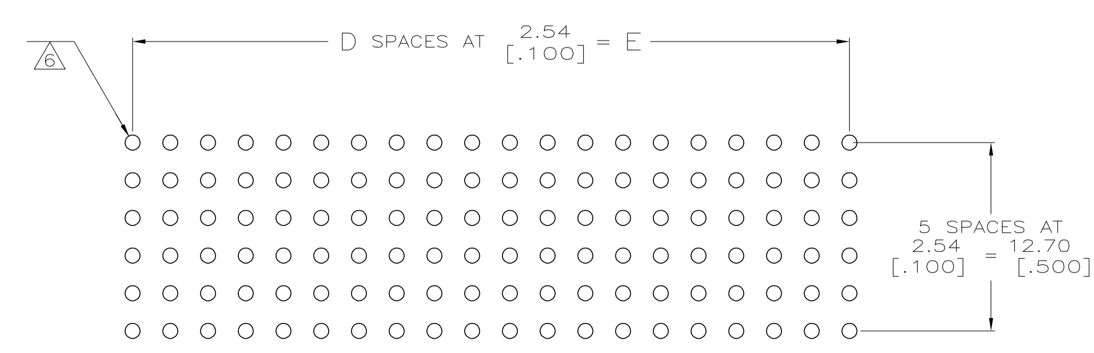
RECOMMENDED P.C BOARD LAYOUT
