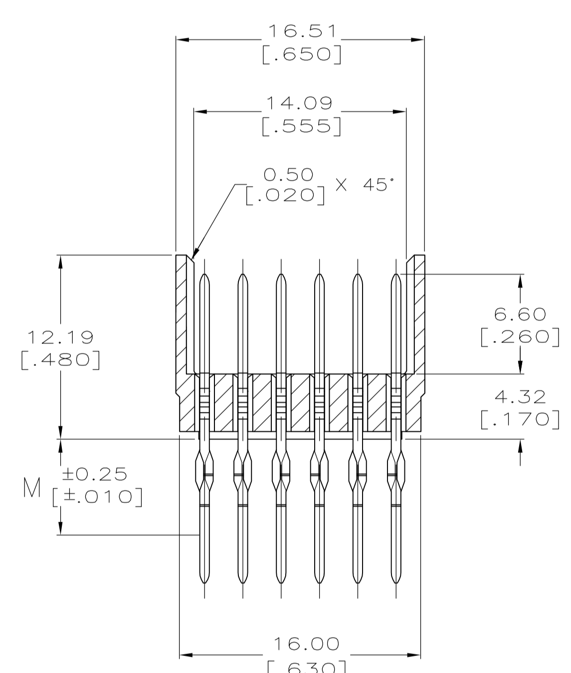
SECTION X-X
